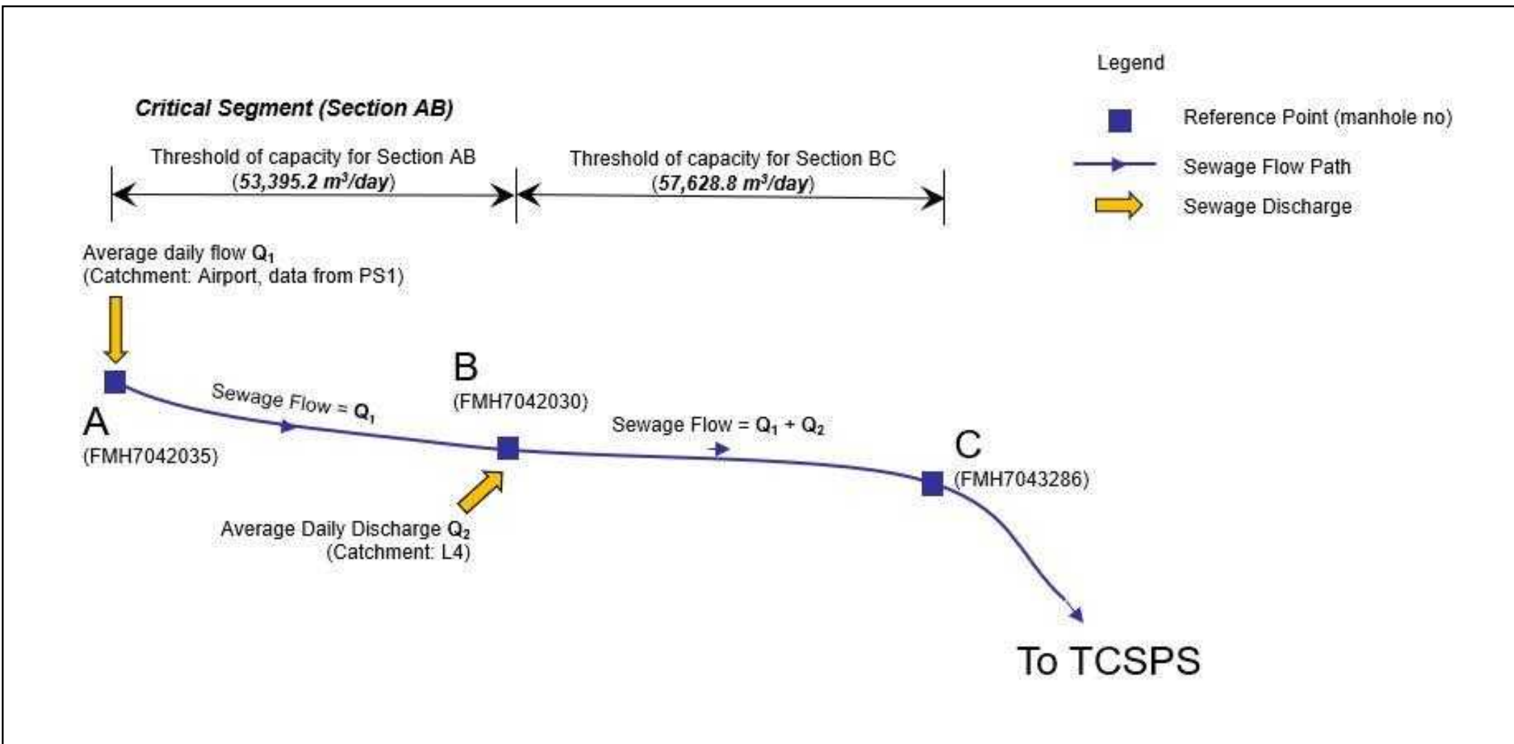
FIGURE 2.8 SCHEMATIC DIAGRAM FOR SEWERAGE SYSTEM FLOW MONITORING
