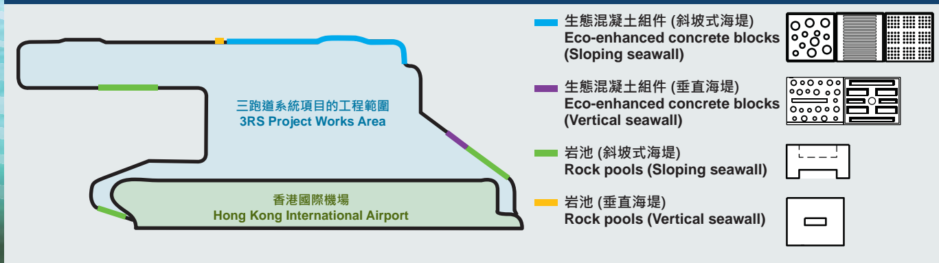
生態混凝土組件及岩池位於不同的潮汐水位，以助潮間帶和潮下帶生物在人工海堤上生長 Eco-enhanced concrete blocks and rock pools are located at different tidal levels to promote colonisation of intertidal and subtidal species on artificial seawalls
