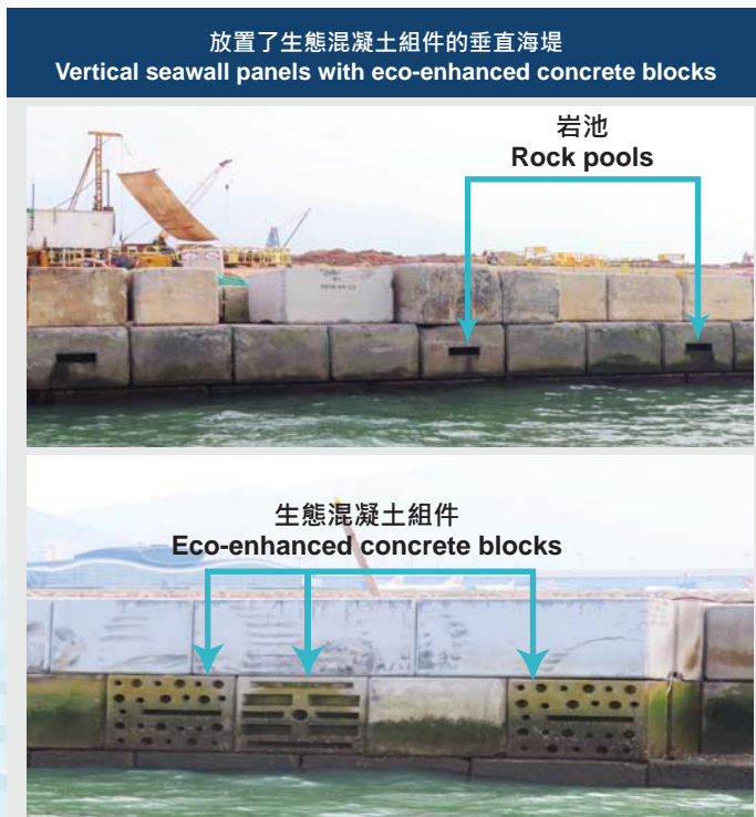
生態混凝土組件及岩池位於不同的潮汐水位，以助潮間帶和潮下帶生物在人工海堤上生長 Eco-enhanced concrete blocks and rock pools are located at different tidal levels to promote colonisation of intertidal and subtidal species on artificial seawalls
