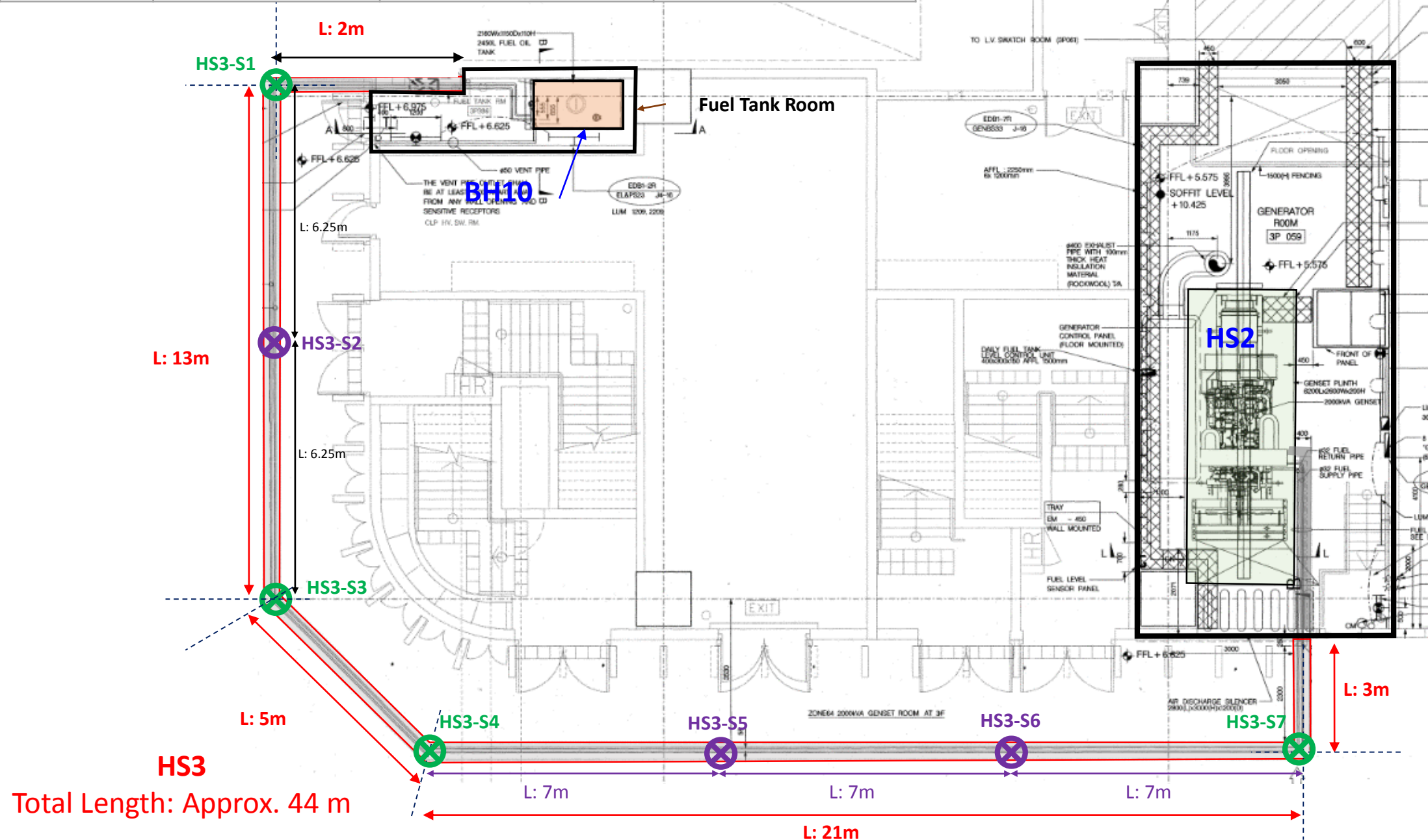
Indicative Sampling Point Selection of Underground Pipeline Trench of Emergency Power Supply System No.4 (i.e. HS3 )
