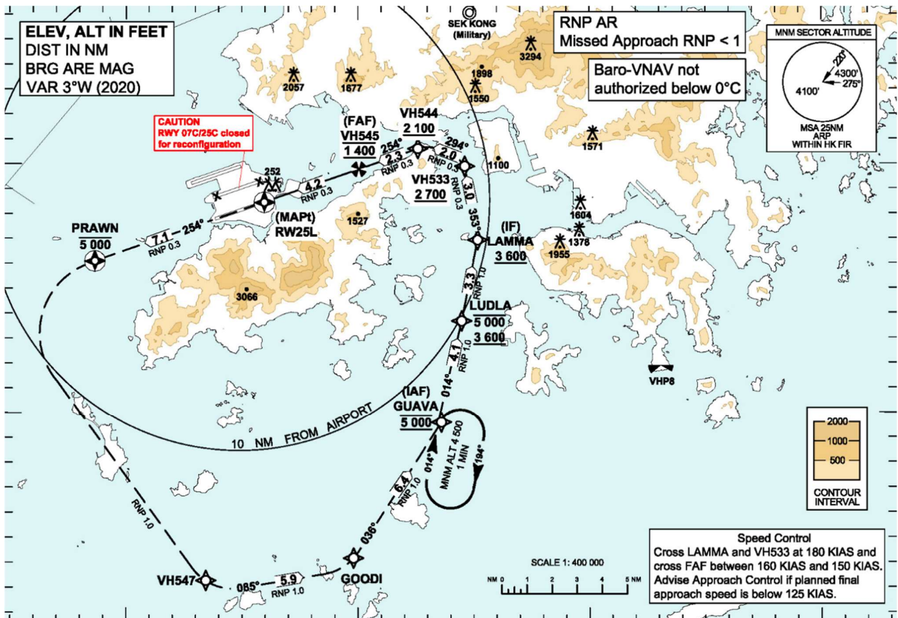
Runway 25L Track 6 RNP-AR Approach path during West Flow in I-2RS operation
