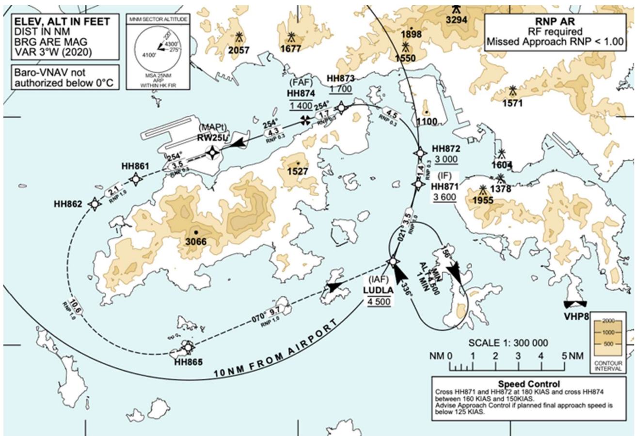
Runway 25L Track 6 RNP-AR Approach path during West Flow in 3RS operation (For contingency use only)
