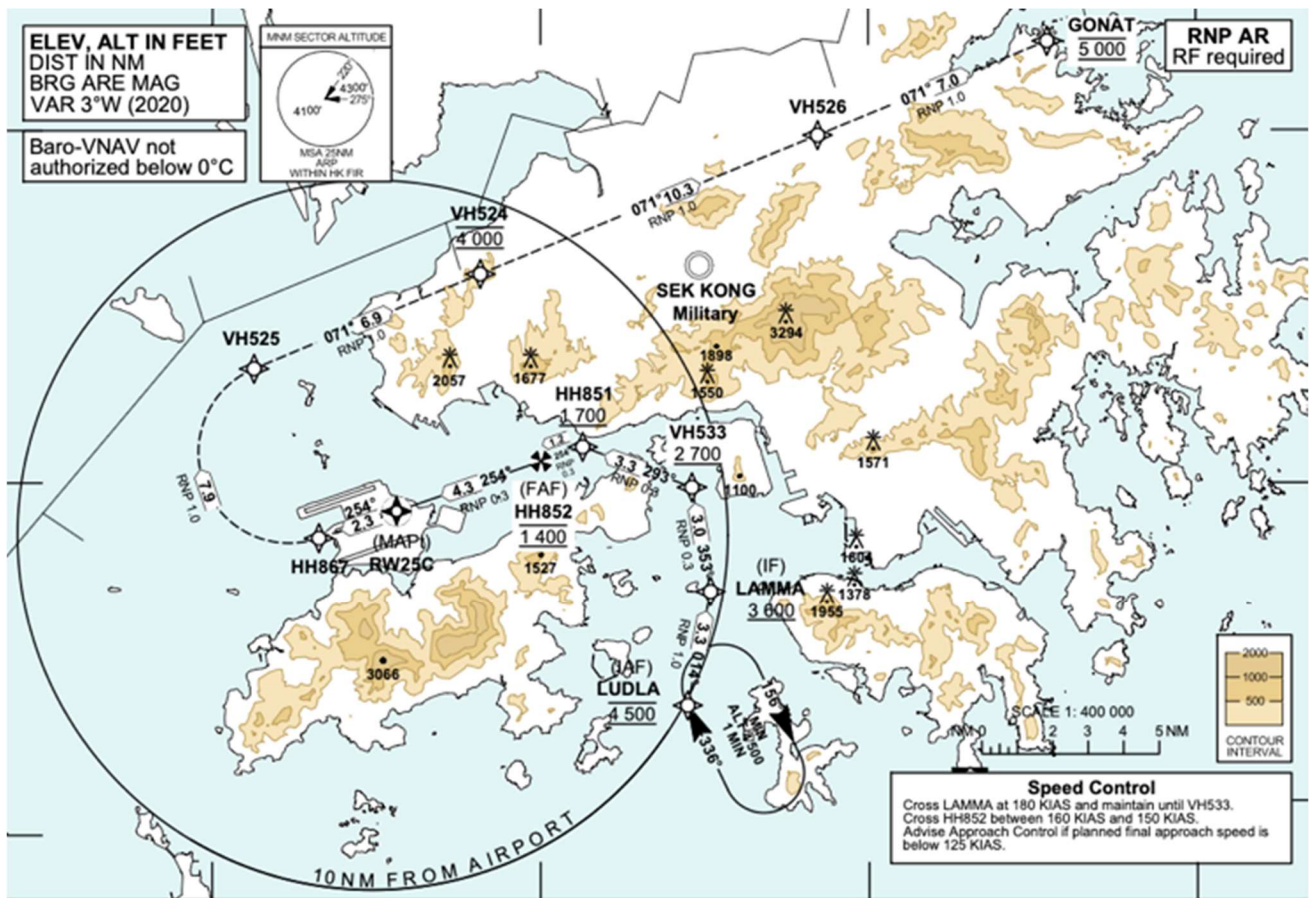
Runway 25C Track 6 RNP-AR Approach path during West Flow in 3RS operation
