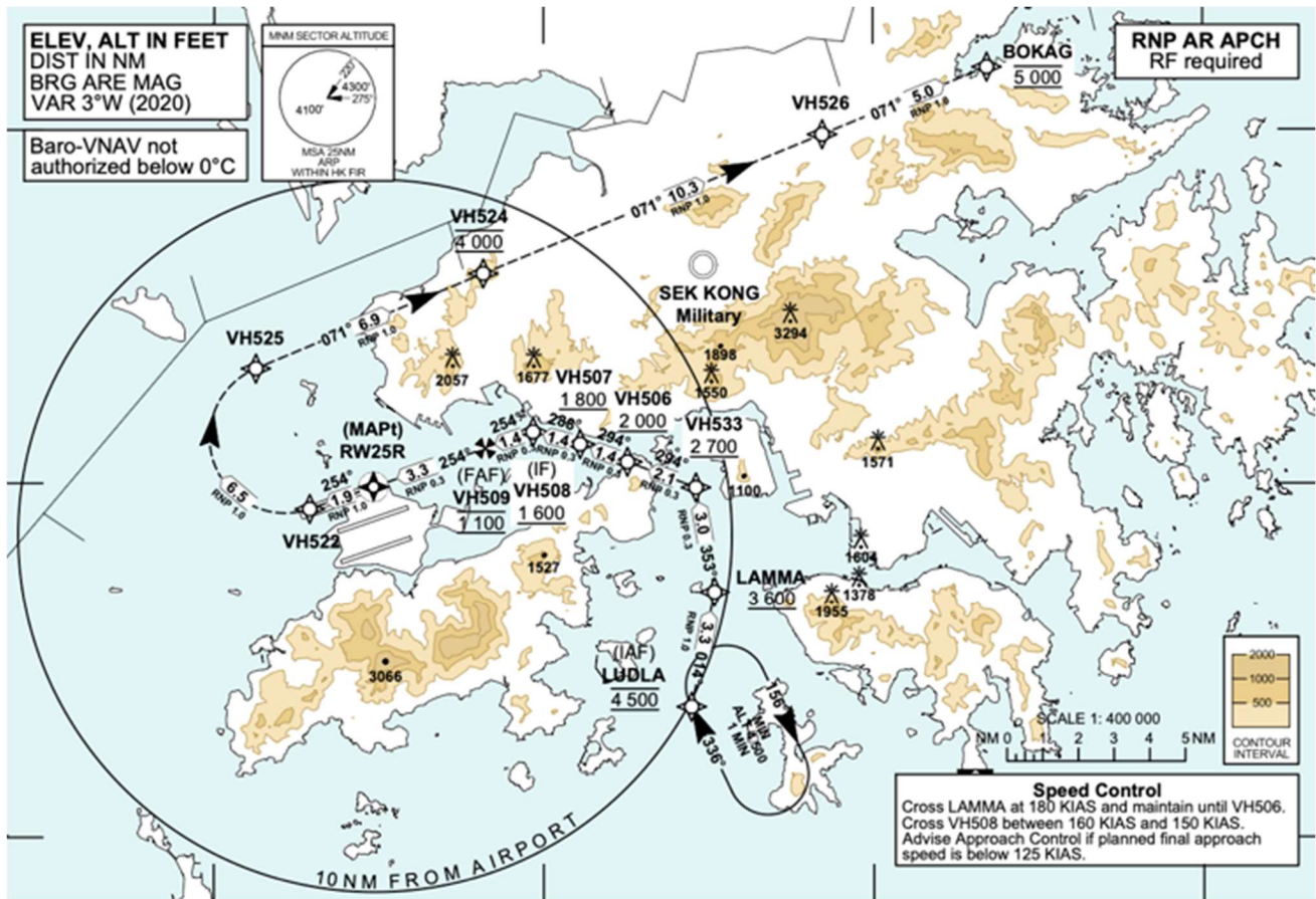
Runway 25R Track 6 RNP-AR Approach path during West Flow in 3RS operation
