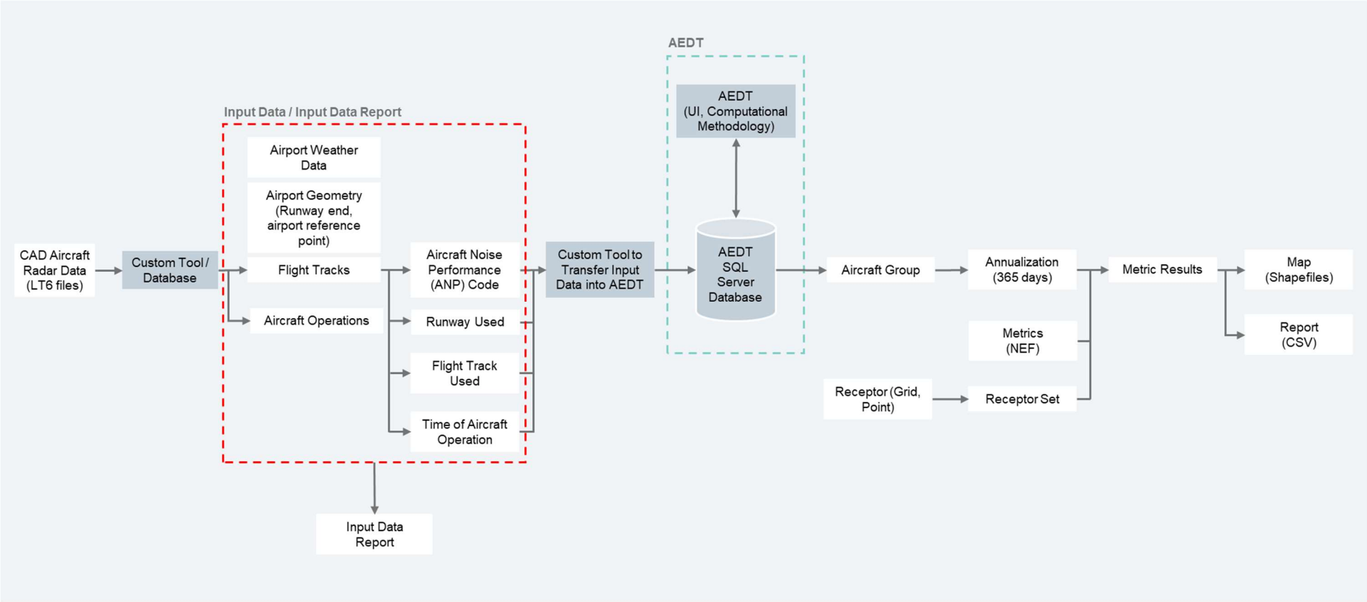
Figure 3.1: Aircraft Noise Modelling Process
